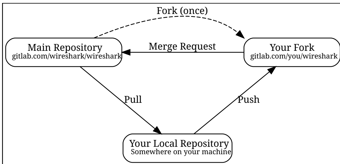
Figure 1. GitLab Workflow
